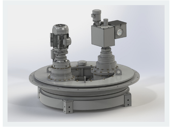
D60-DF-D60 retrofit for Eimco C60/C72P on a Ø180 ft industrial solids contact clarifier
