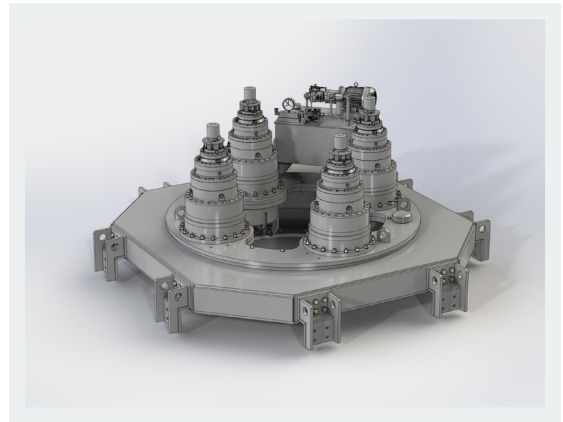
D80-EH4 retrofit for Dorr-Oliver 122S3 on a Ø250 ft pulp and paper effluent
